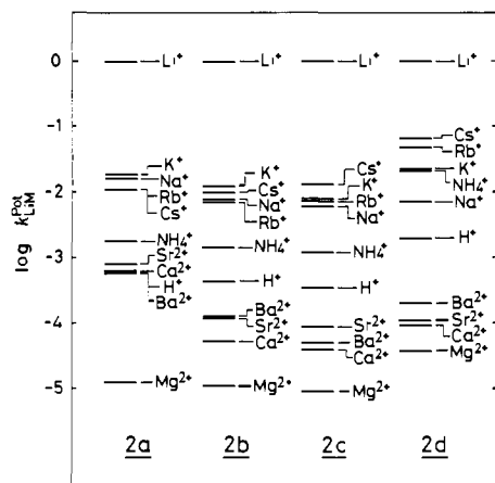
Figure 4. Selectivity coefficients \log k_{LiM}^{Pot} for PVC membranes containing lipophilic crown-4 derivatives 2a–2d .
