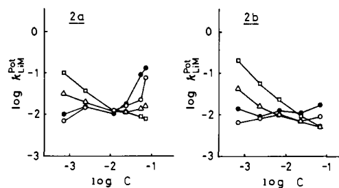
Figure 5. Dependence of \log k_{LiM}^{Pot} values on crown ether concentration in PVC membranes of 2a and 2b . M: Na^+ (○), K^+ (●), Rb^+ (△), Cs^+ (□).
